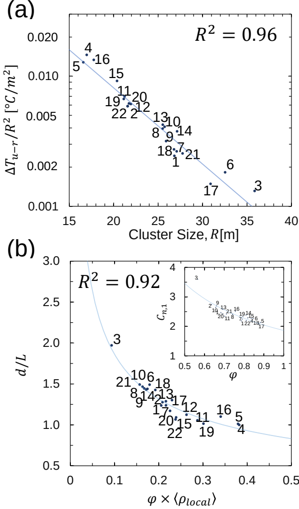
FIG. 3. (color online) City texture parameters [22] for group A cities. (a) Relationship between \Delta T_{u-r} and the cluster size R . Measured and model-predicted relationship of city texture, obtained from the upper limit of the integral of the first peak of g(r) , shows a strong negative correlation captured with a power law. (b) Power-law correlation of the form y = a \times x^b , where a = 0.59 and b = -0.5 , between the ratio of average distance between buildings d (obtained using R = 1.5d ) and building size L , and the product of the local Mermin order parameter, \phi , and local density, \langle \rho_{local} \rangle . The inset shows an inverse relationship of the form y = 1.8/x between the number of local neighboring buildings, C_{n,1} and \phi .
