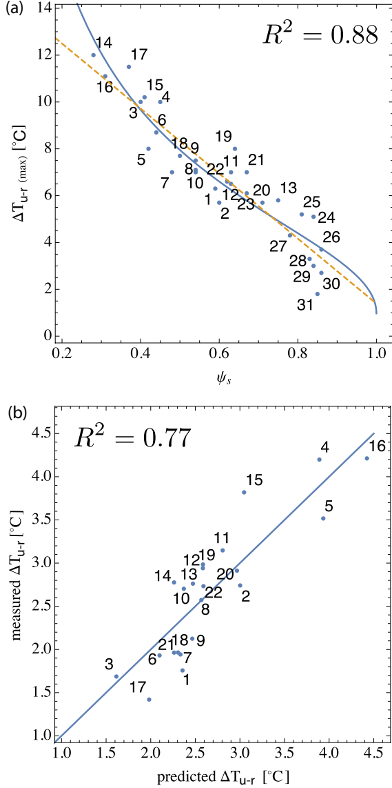
FIG. 4. (color online) Relationship between measured and model-predicted \Delta T_{u-r} . (a) maximal \Delta T of group B cities as a function of the sky view factor \psi_s from Oke [31] together with the linear fit of Oke (dashed line) and the fit to our model (solid curve), from Eq. (2). Numbers in the figure correspond to cities analyzed by Oke [31]. (b) Comparison of measured and predicted \Delta T_{u-r} for group A cities using Eq. (1).
