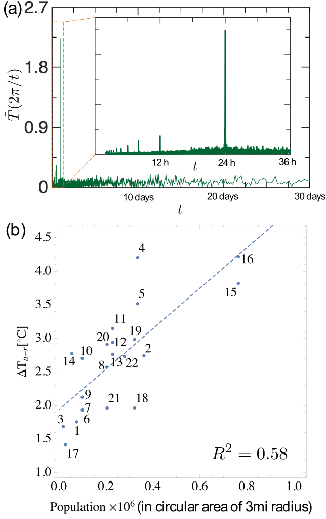
FIG. 1. (color online) Night-time UHI intensity from Fourier analysis of temperature time series and population influences. (a) Fourier transformed temperature time series for Boston, MA. (b) Relationship between \Delta T_{u-r} s and population within 3-mile radius from urban weather stations.
