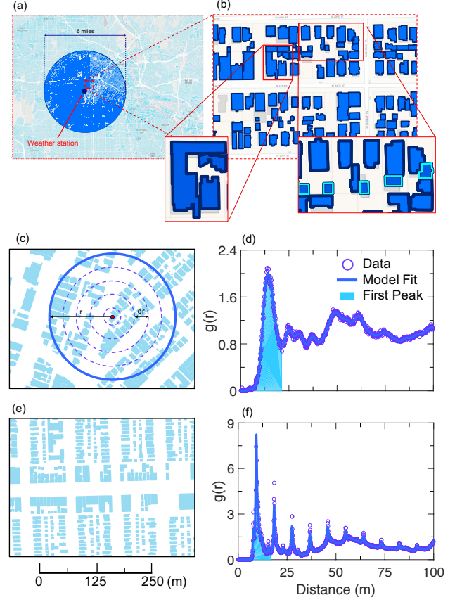
FIG. 2. (color online) Radial distribution function, g(r) , for city texture that depicts visualization of data editing, analysis and results. (a) Buildings within a 3-mile radius of an urban weather station are extracted. (b) Any buildings that share a wall are merged and any unoccupied buildings (i.e. garages) are removed from the sample of buildings transformed into a set of single points using buildings' 2-D center of mass. (c) City texture of Los Angeles, CA showing a comparable absence of order of buildings caused by dispersed streets captured by (d) the smooth and outspread peaks in g(r) , which generally are characteristic properties of liquids. (e) City texture of Chicago, IL showing order of buildings and periodicity reflected in (f) the sharp and narrow peaks of g(r) , characteristics that are known to be the hallmark of highly ordered and stable crystalline materials.
